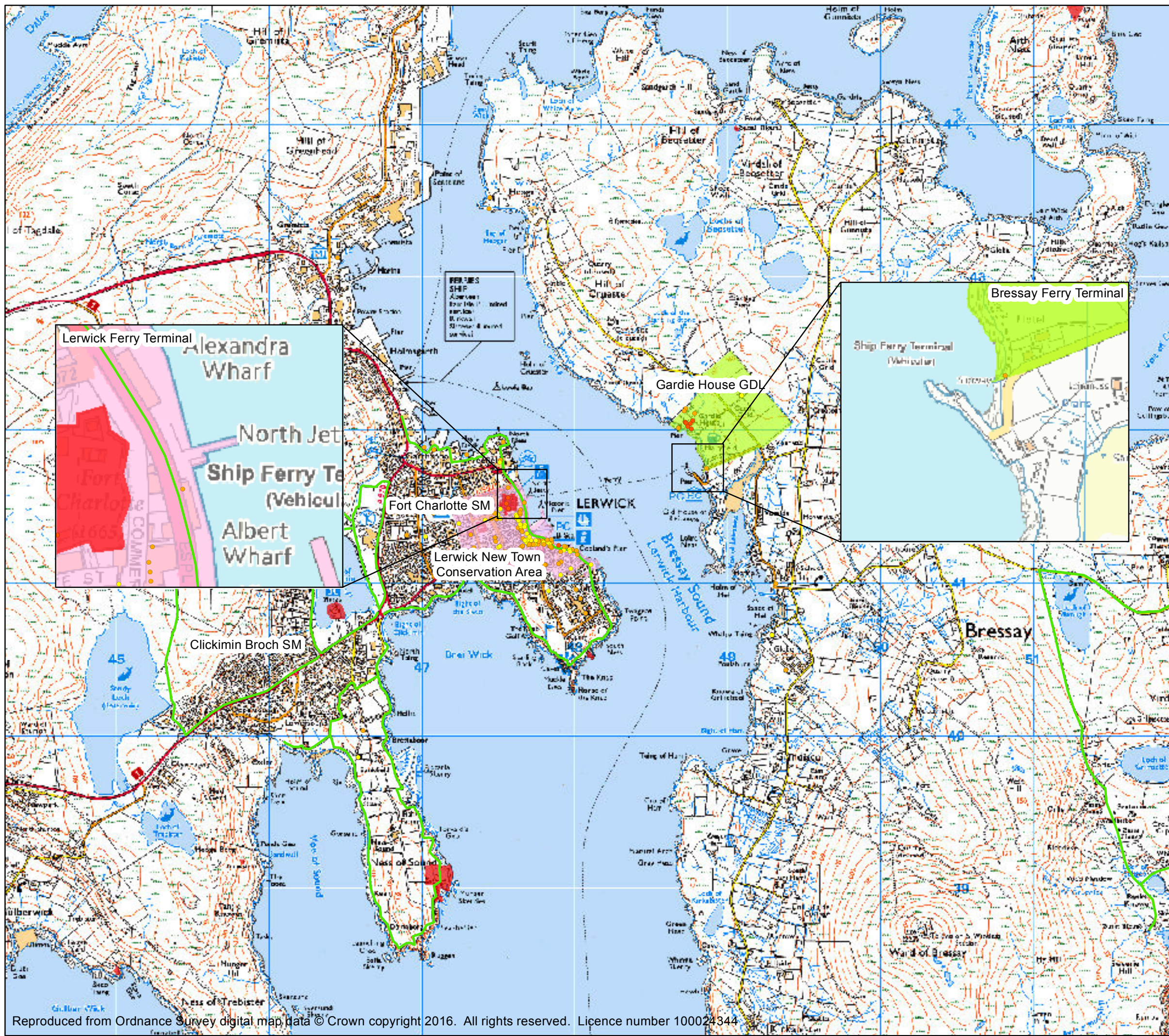
Figure 1: Environmental Constraints Plan Lerwick and Bressay Ferry Terminals
