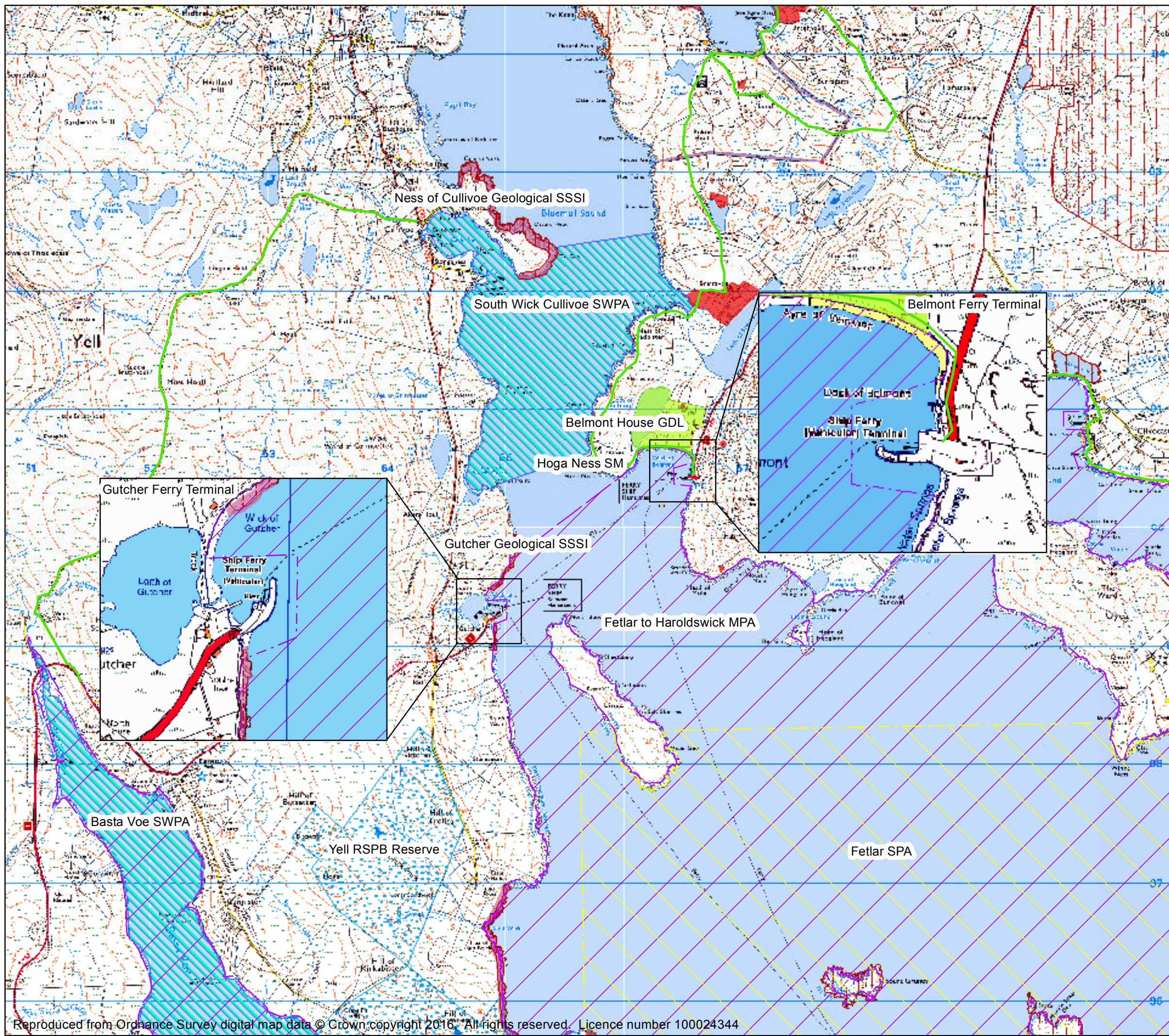
Figure 3: Environmental Constraints Plan Gutcher and Belmont Ferry Terminals
