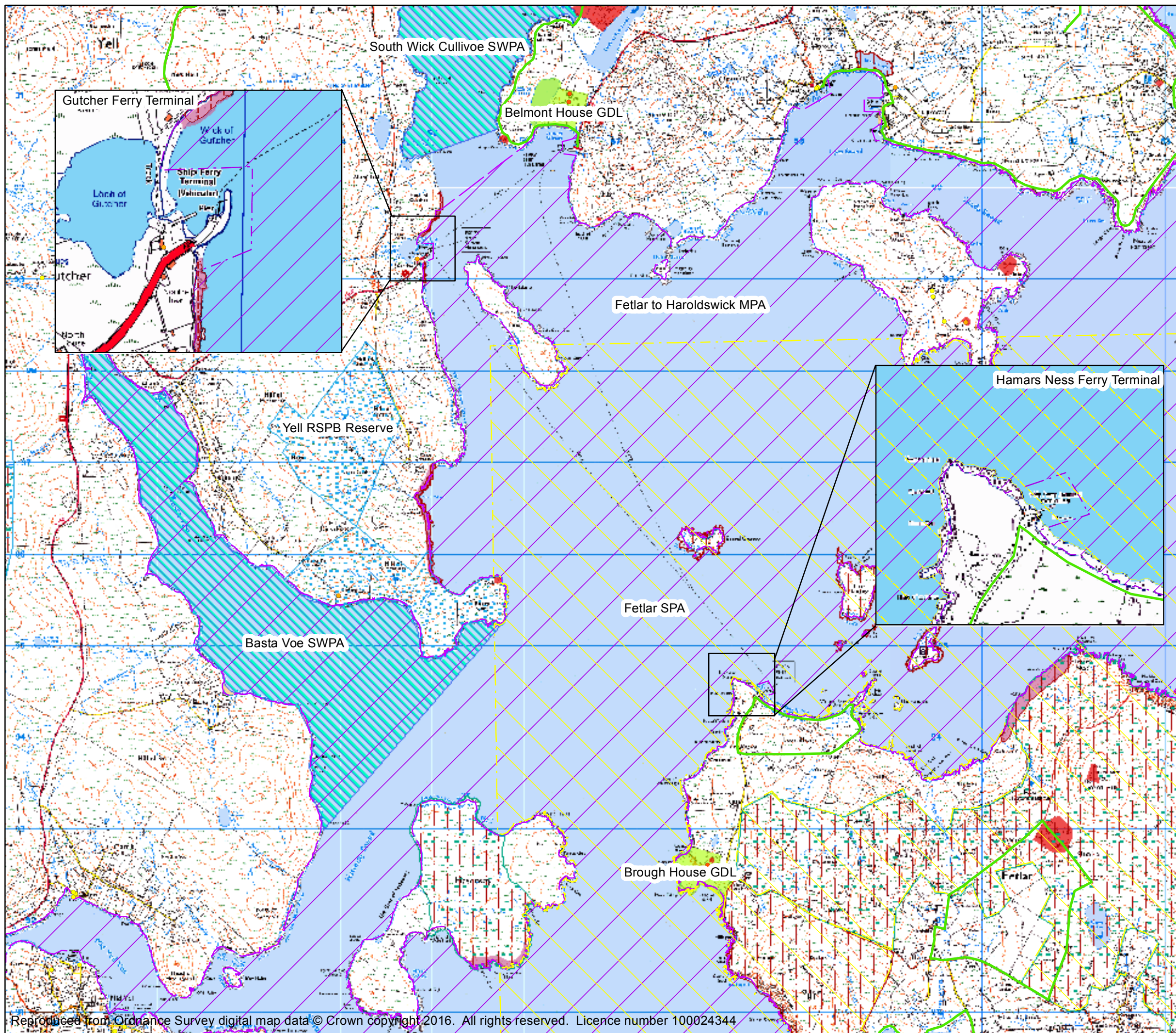
Figure 4: Environmental Constraints Plan Gutcher and Hamars Ness Ferry Terminals
