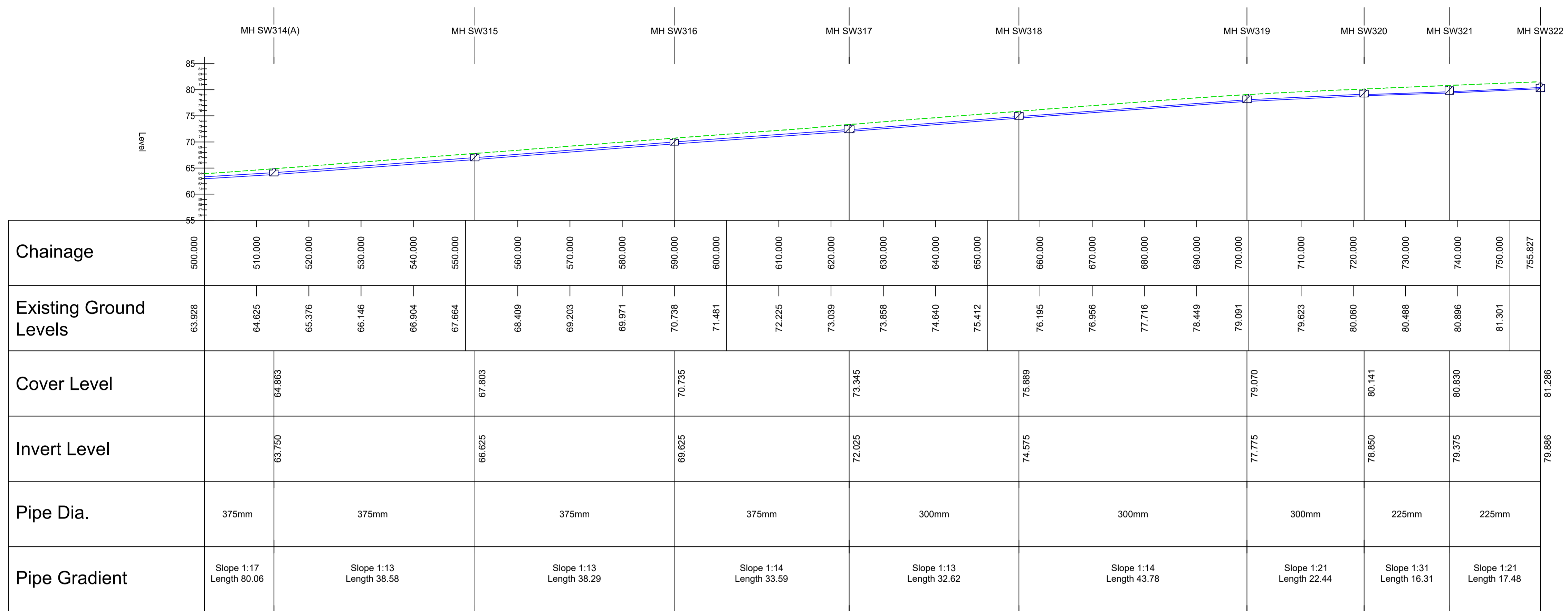
LONG SECTION THROUGH SPINE ROAD SURFACE WATER DRAINAGE MANHOLES SW315 to SW322 HORZ SCALE 1:500; VERT SCALE 1:500
