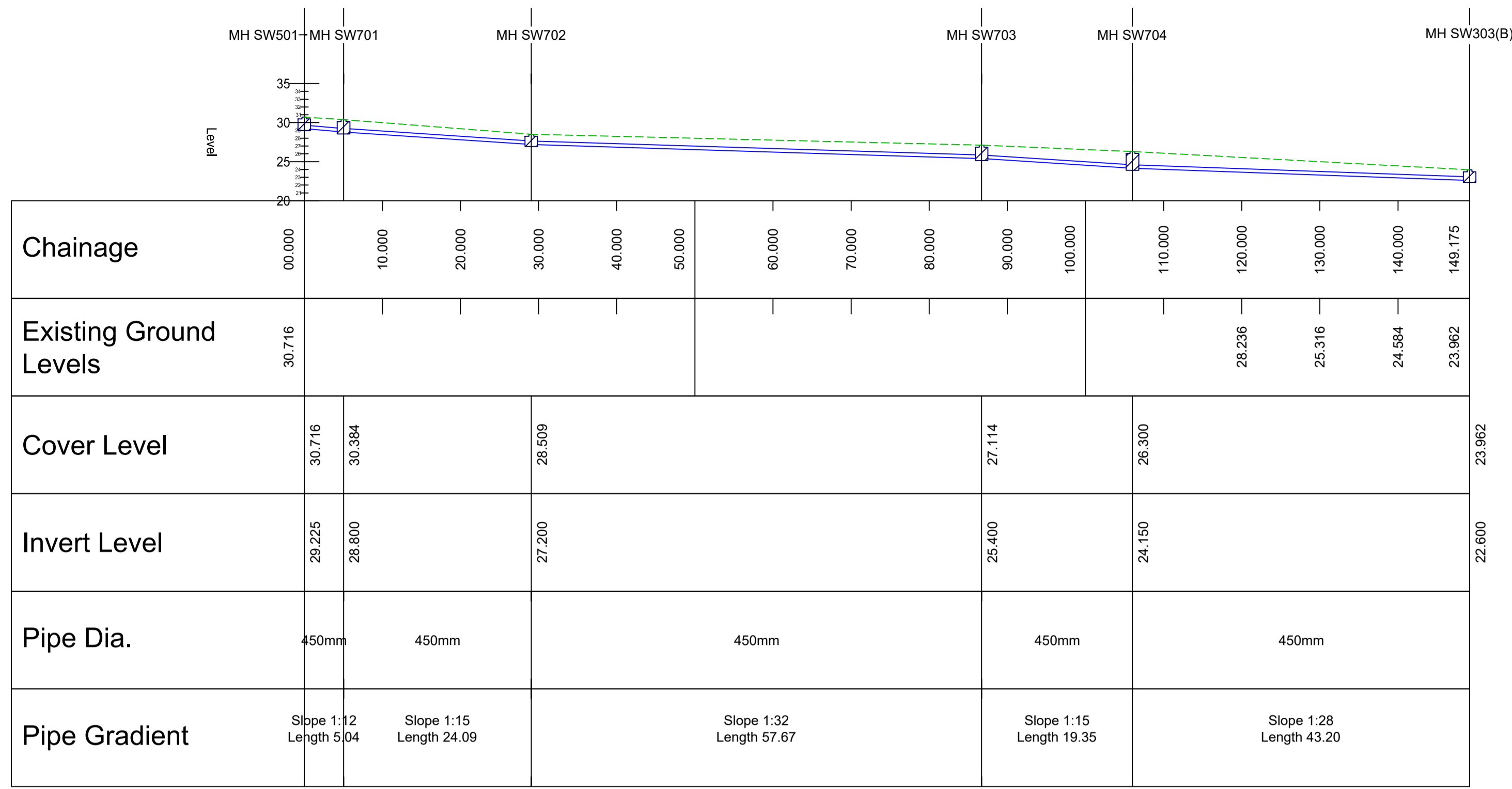
LONG SECTION THROUGH UPPER SUDS AREA SURFACE WATER DRAINAGE MANHOLES SW501 to SW303(B) HORZ SCALE 1:500; VERT SCALE 1:500
