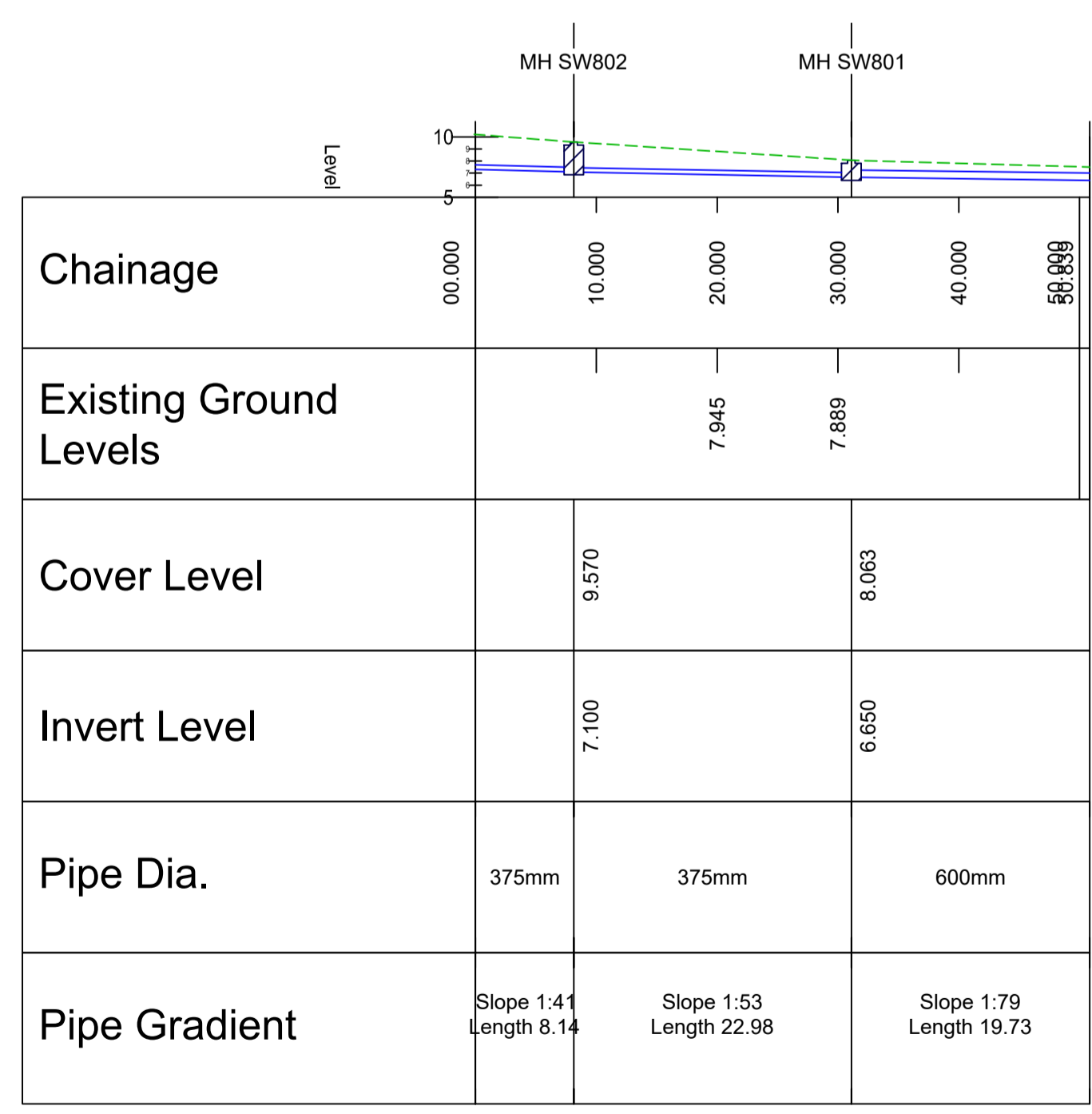
LONG SECTION THROUGH LOWER SUDS AREA SURFACE WATER DRAINAGE MANHOLES SW802 to SW801 HORZ SCALE 1:500; VERT SCALE 1:500
