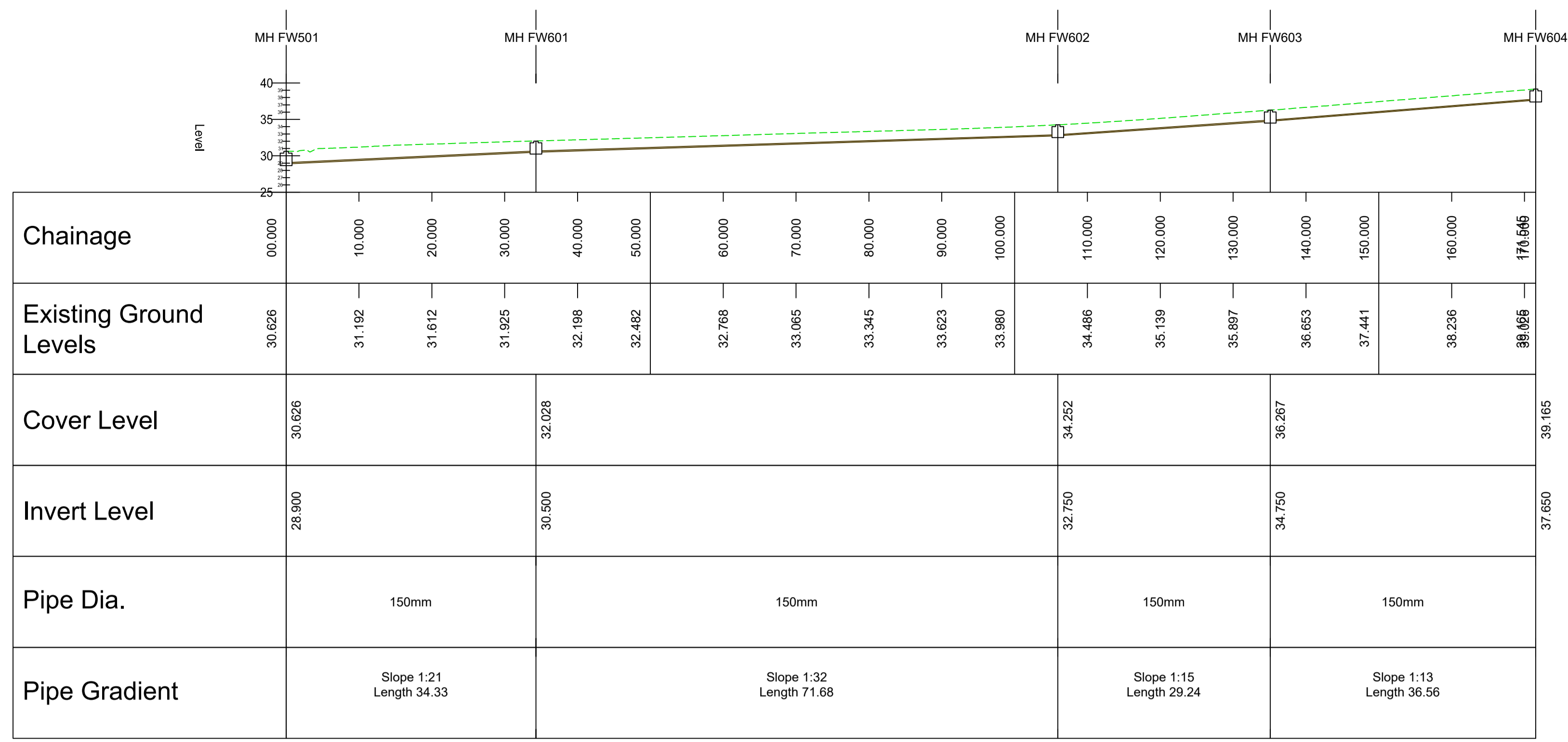
LONG SECTION THROUGH UPPER ESCARPMENT ROAD FOUL SEWER DRAINAGE MANHOLES FW501 to FW604 HORZ SCALE 1:500; VERT SCALE 1:500
