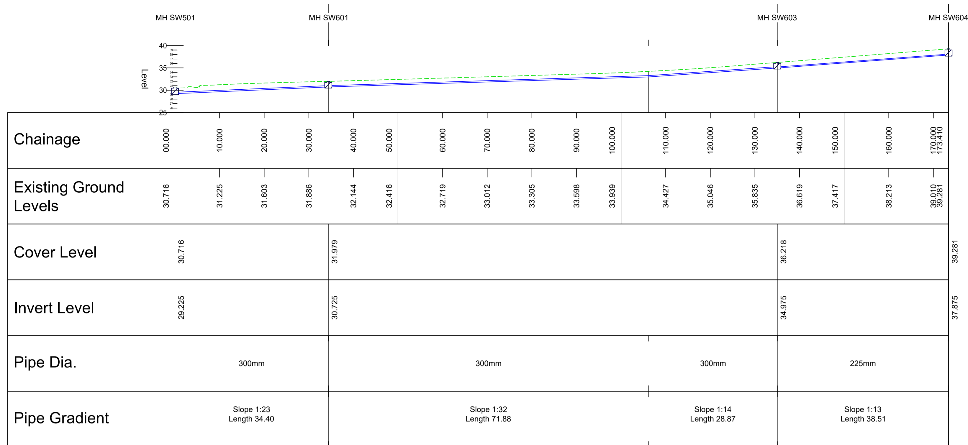
LONG SECTION THROUGH UPPER ESCARPMENT ROAD SURFACE WATER DRAINAGE MANHOLES SW501 to SW504 HORZ SCALE 1:500; VERT SCALE 1:500
