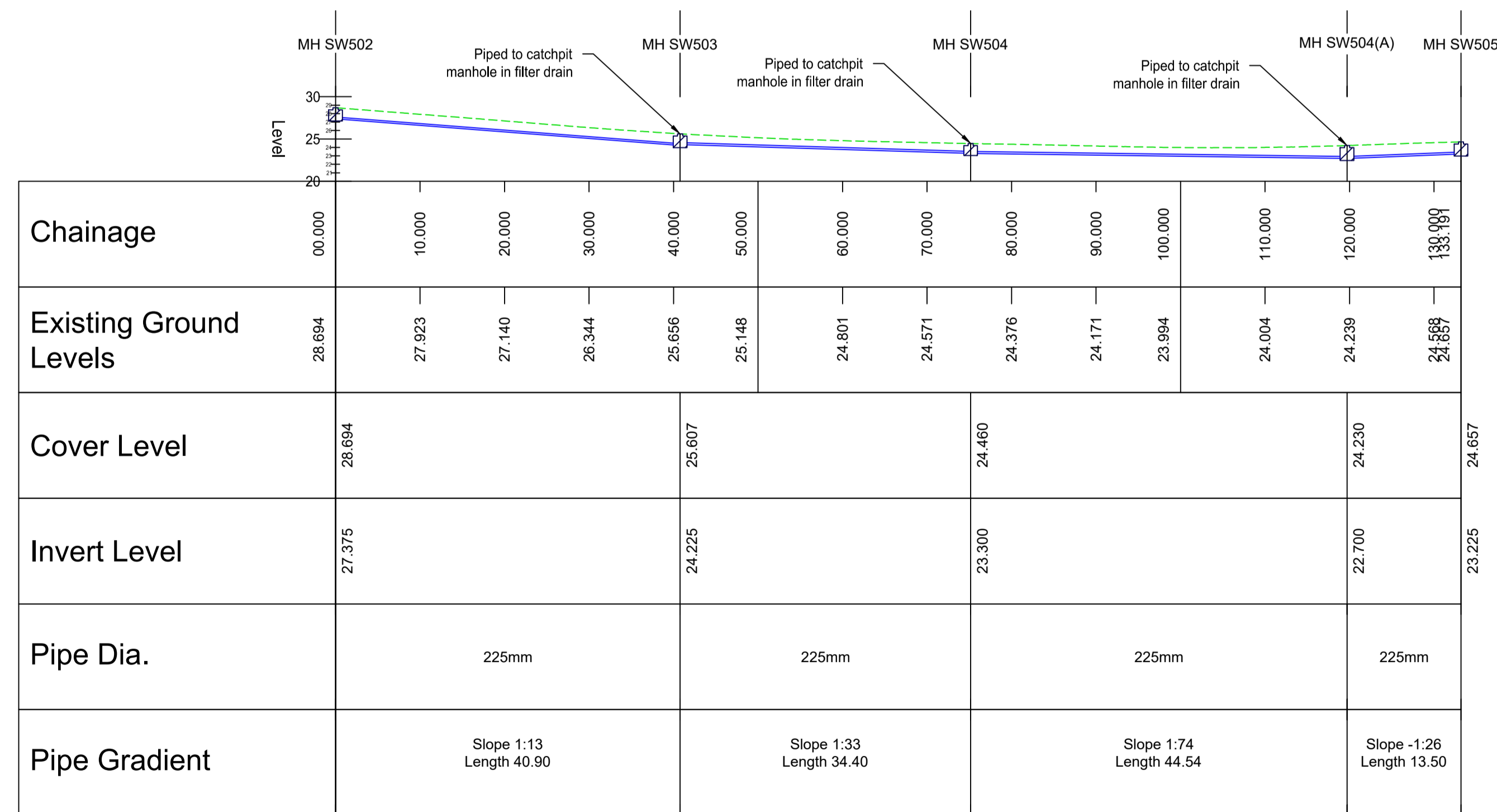
LONG SECTION THROUGH UPPER ESCARPMENT ROAD SURFACE WATER DRAINAGE MANHOLES SW502 to SW504 HORZ SCALE 1:500; VERT SCALE 1:500
