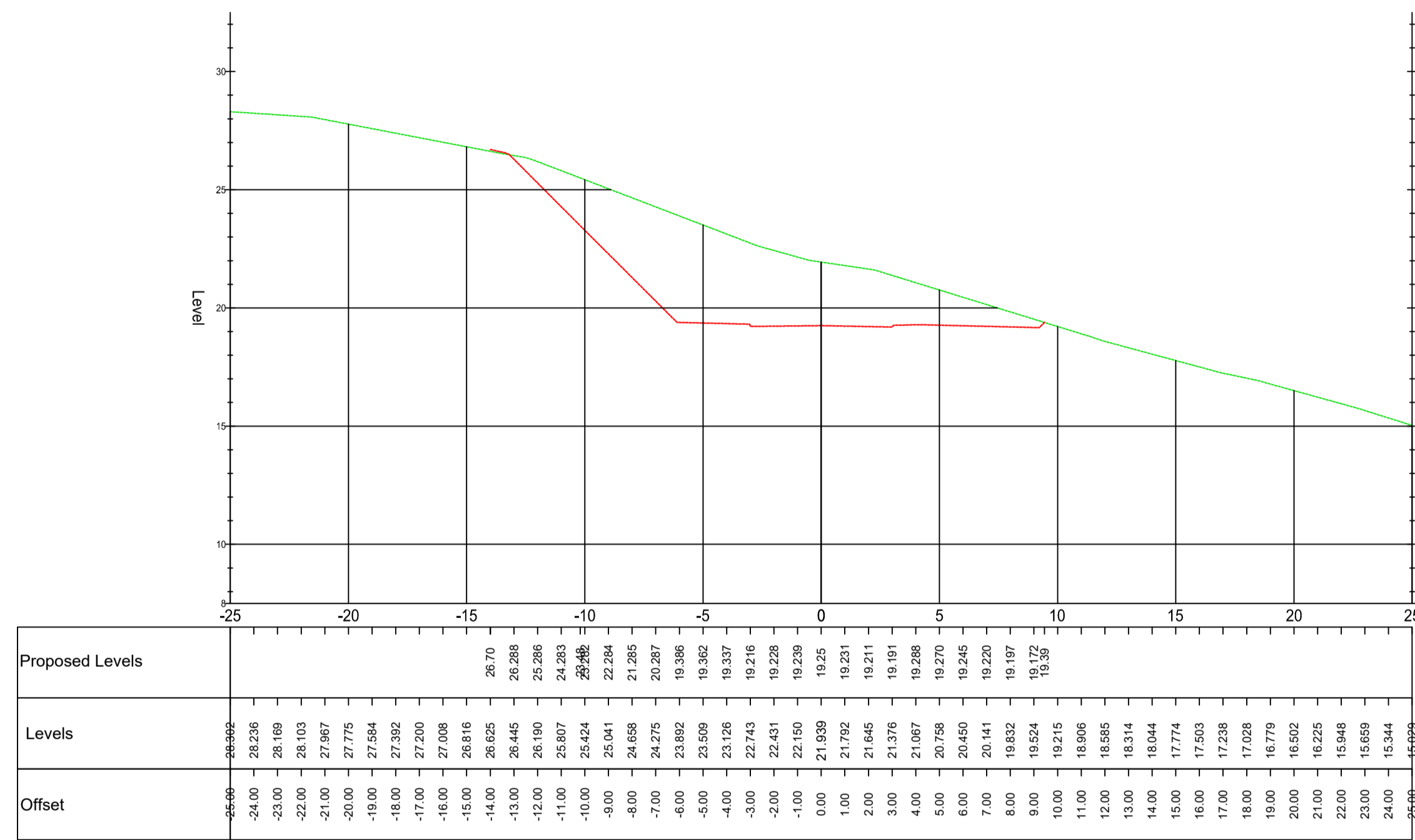
CROSS SECTION THROUGH SPINE ROAD - CHAINAGE 20m HORZ SCALE 1:200; VERT SCALE 1:200
