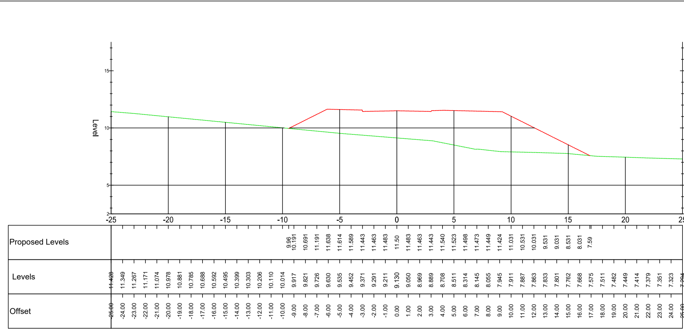
CROSS SECTION THROUGH SPINE ROAD - CHAINAGE 20m HORZ SCALE 1:200; VERT SCALE 1:200
