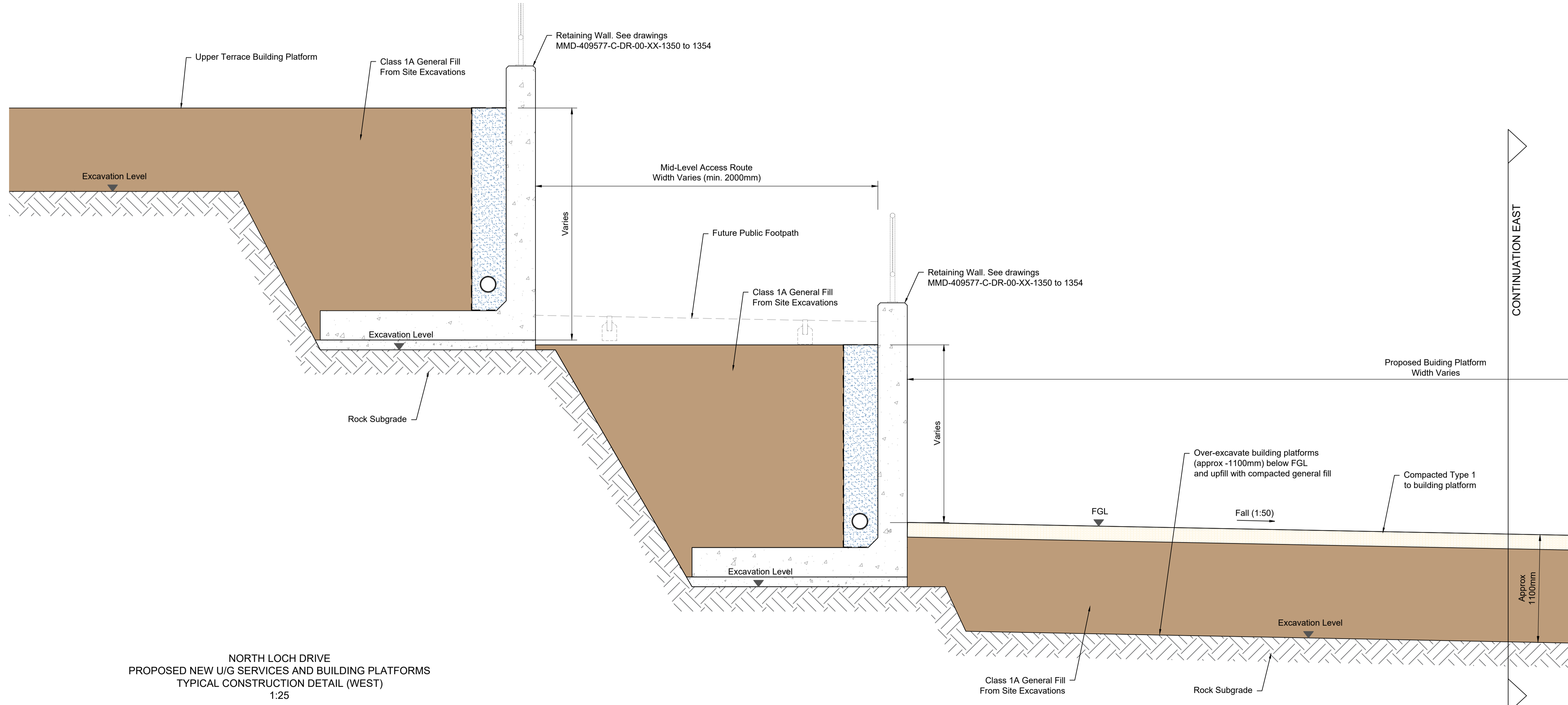
NORTH LOCH DRIVE PROPOSED NEW U/G SERVICES AND BUILDING PLATFORMS TYPICAL CONSTRUCTION DETAIL (EAST) 1:25
