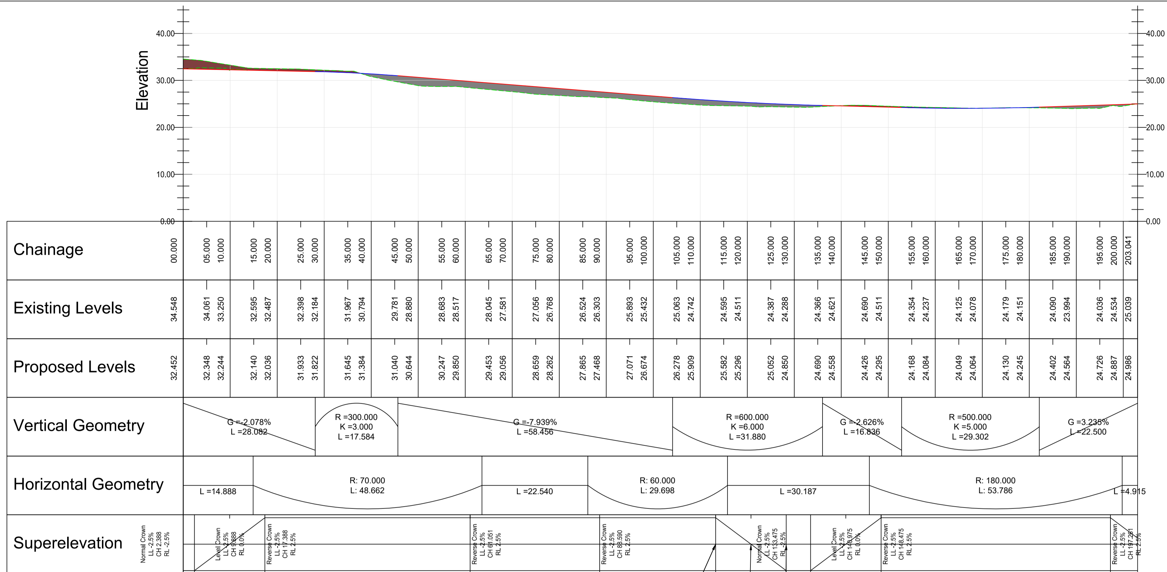
LONG SECTION THROUGH ESCARPMENT ROAD LOWER CHAINAGES 0m - 203.041m HORZ SCALE 1:500; VERT SCALE 1:500
