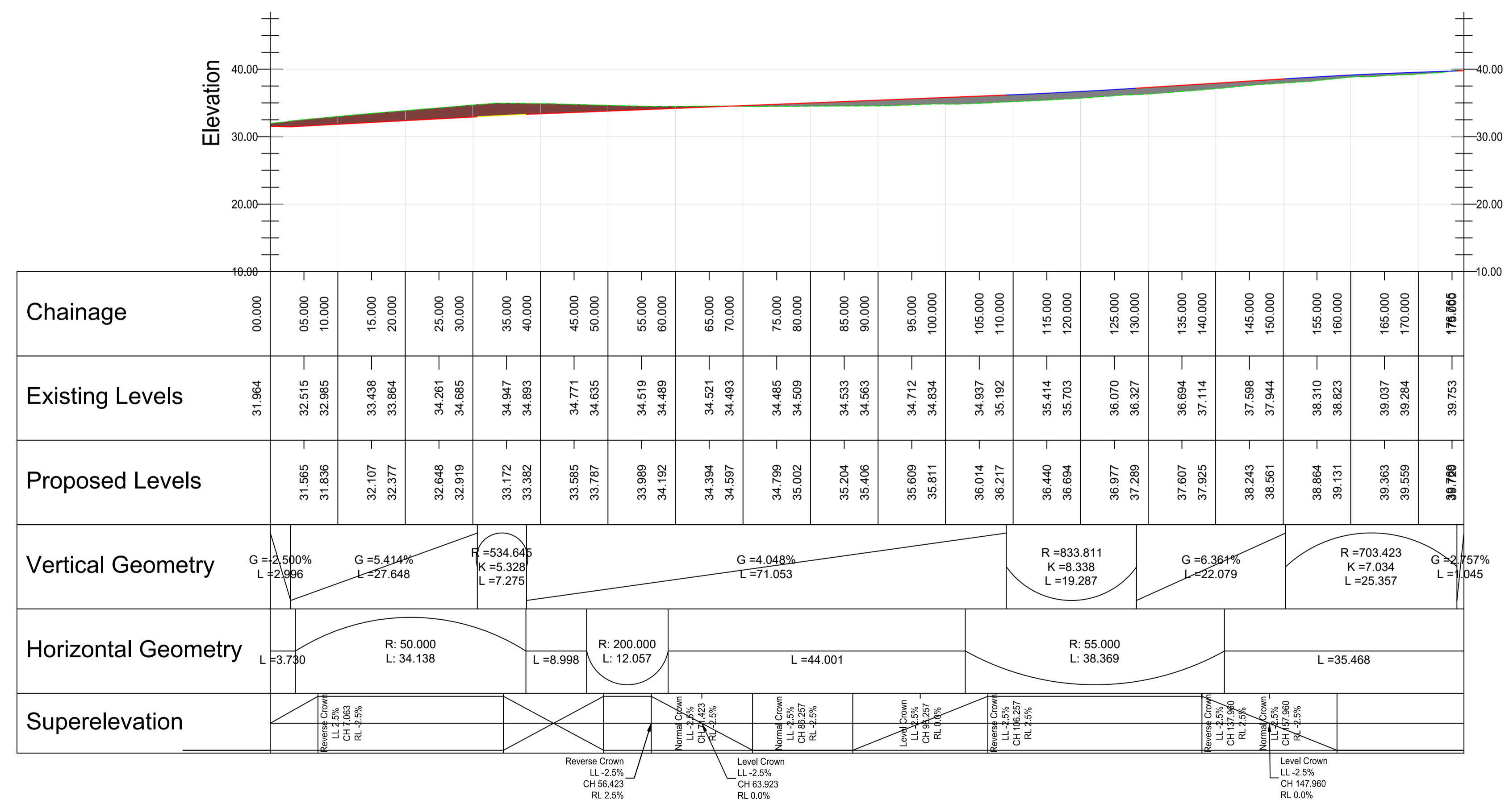
LONG SECTION THROUGH ESCARPMENT ROAD UPPER CHAINAGES 0m - 176.765m HORZ SCALE 1:500; VERT SCALE 1:500
