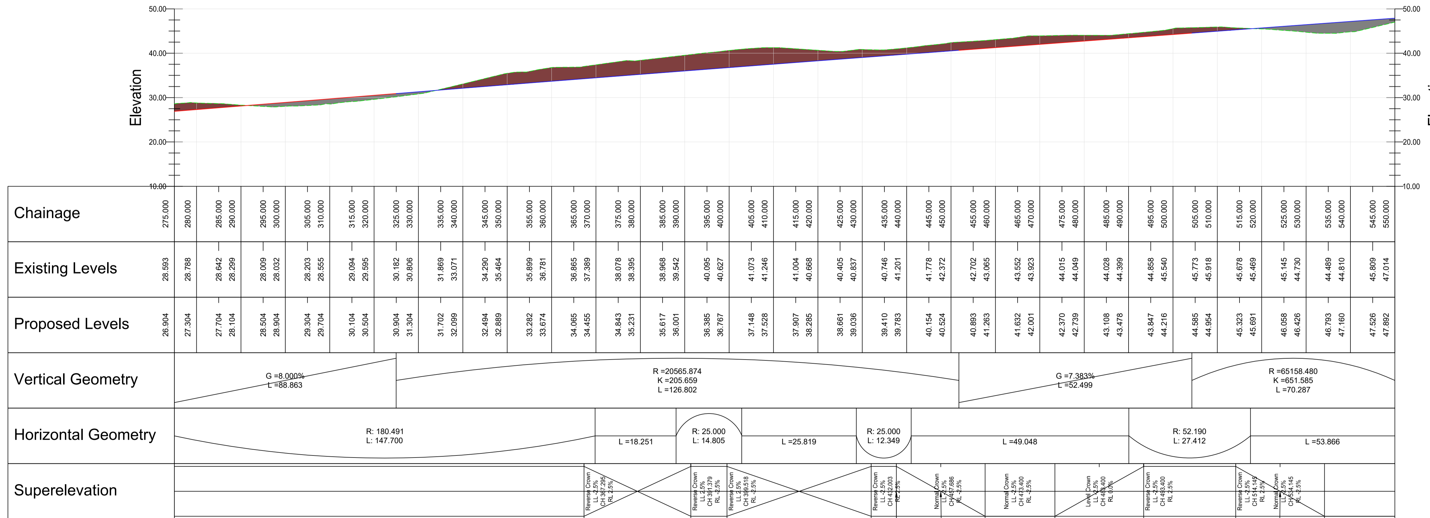
LONG SECTION THROUGH SPINE ROAD CHAINAGES 275m - 550m HORZ SCALE 1:500; VERT SCALE 1:500
